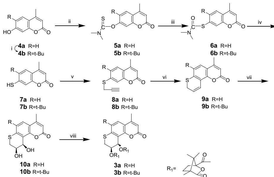
Scheme 1. Reagents and conditions: (i) t -BuOH, H 3 PO 4 /P 2 O 5 ; (ii) dimethylthiocarbamoyl chloride, DMAP/CH 2 Cl 2 ; (iii) heating; (iv) (1) NaOCH 3 /MeOH, (2) HCl; (v) 3-bromo-1-propyne, K 2 CO 3 , KI, acetone/N 2 ; (vi) N,N -diethylaniline, reflux; (vii) (1) K 2 OsO 2 (OH) 4 , K 3 Fe(CN) 6 , (DHQ) 2 -PHAL, K 2 CO 3 , (2) Na 2 SO 3 ; (viii) camphanic chloride, DMAP/CH 2 Cl 2 .
